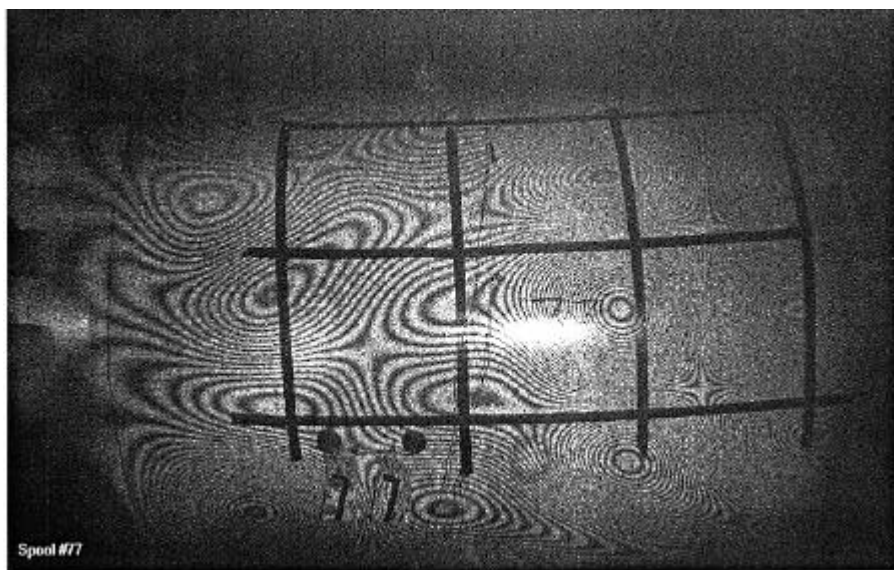
Figure 6. Transient phenomena similar to a shock wave progressing through the spool. This is seen as a increase in displacement on the right side (up stream) region denoted by increase in fringe density
