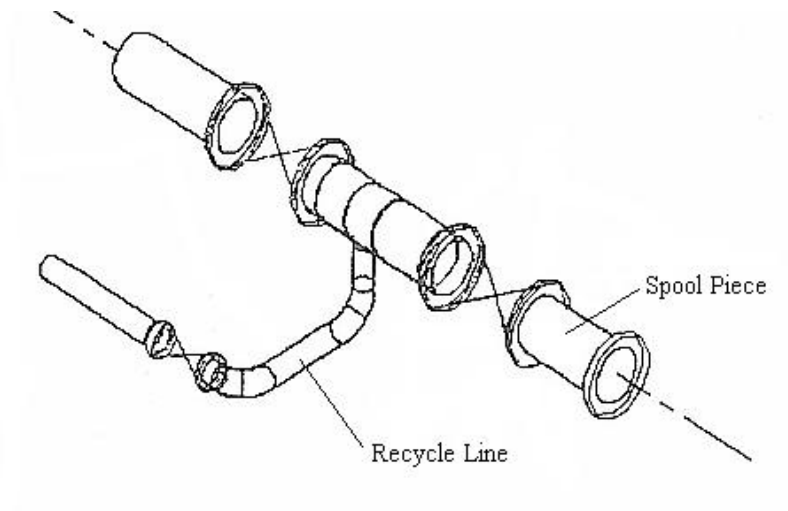
Figure 1. Gas conveying piping elements, the layout of the piping arrangement. The turbine is located to the right of the spool
